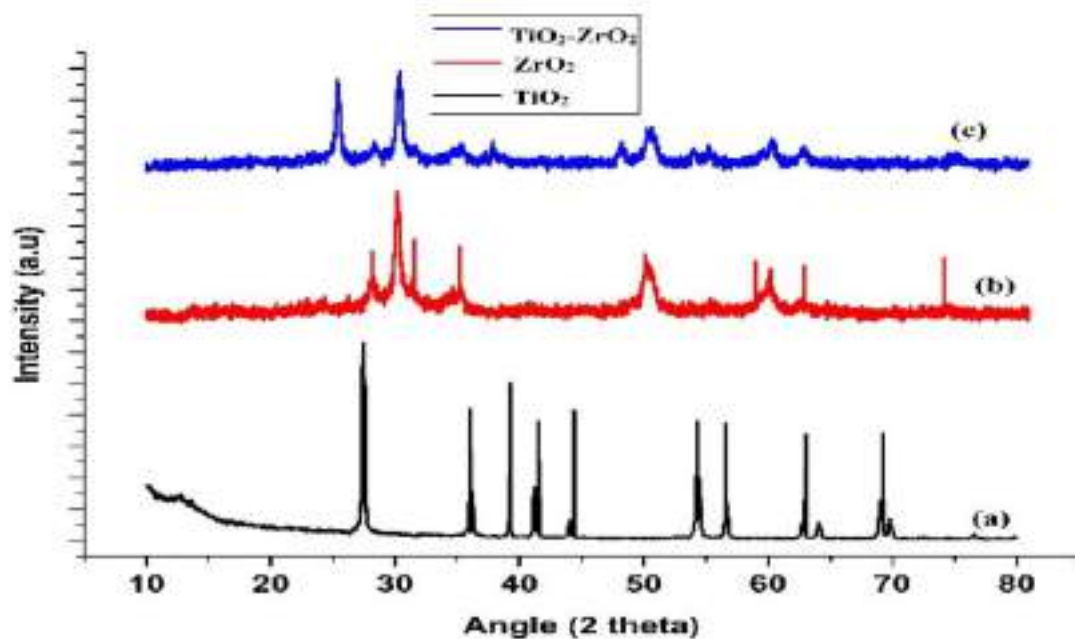
Fig. 2: XRD pattern of (a) \text{TiO}_2 (b) \text{ZrO}_2 (c) mixed phase \text{TiO}_2\text{-ZrO}_2 nanocomposite. 30
