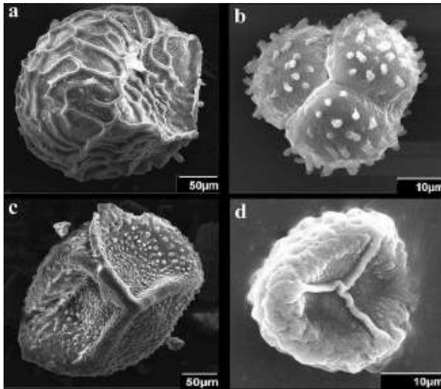
Figure 3. Megaspore and microspore micromorphology. a,b: Selaginella ganguliana R.D.Dixit; c,d: Selaginella tenera (Hook. & Grev.) Spring ( a,c: Megaspore; b,d: Microspore)
