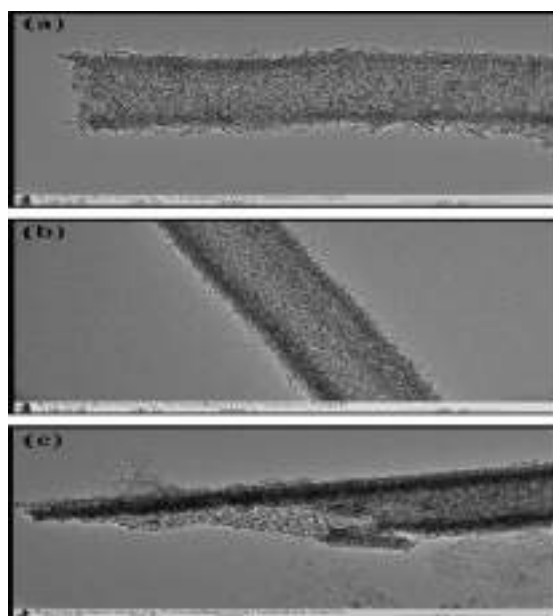
Fig. 4. TEM analyses of (a) \text{TiO}_2 nanotube, (b) \text{ZrO}_2 nanotube and (c) \text{TiO}_2/\text{ZrO}_2 composite nanotube. 40
